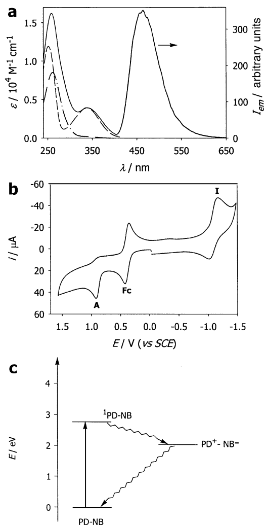
Fig. 2 (a) Absorption (298 K) and emission (77 K) spectra of the PD-NB dyad (full line) and absorption spectra of the PD (dashed line) and nitrobenzene (dashed-dotted line) components in acetonitrile. (b) Cyclic voltammogram of the PD-NB dyad in acetonitrile-TEAPF 6 solution. (c) Energy level diagram for the PD-NB dyad in acetonitrile solution at room temperature.
