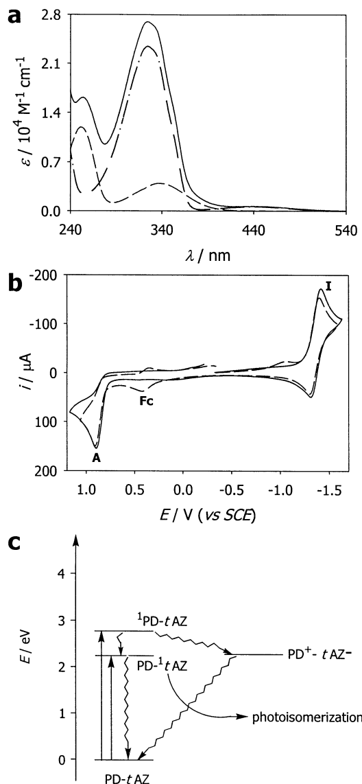
Fig. 4 (a) Absorption spectra of the PD- t AZ dyad (full line) and the PD (dashed line) and t MeAZ (dashed-dotted line) components in acetonitrile. (b) Cyclic voltammogram of the PD- t AZ (full line) and PD- c AZ (dashed line) dyads in acetonitrile-TEAPF 6 solution. (c) Energy level diagram for the PD- t AZ dyad.
