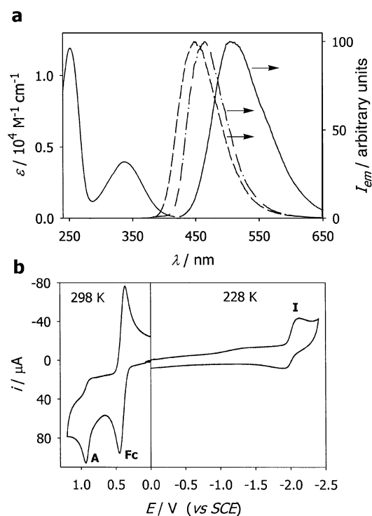
Fig. 1 (a) Full line: absorption and fluorescence spectra in acetonitrile solution at 298 K of 5-dimethylaminonaphthalene- N -propyl-1-sulphonamide (PD). The fluorescence spectra in butyronitrile at 77 K (dashed-dotted line) and in cyclohexane at 298 K (dashed line) are also shown. (b) Cyclic voltammogram of PD in acetonitrile- \text{TEAPF}_6 solution.
