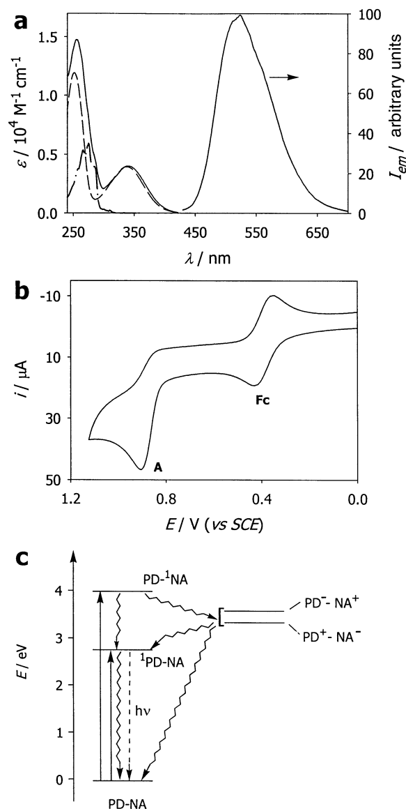
Fig. 3 (a) Absorption and emission spectra of the PD-NA dyad (full line) and absorption spectra of the PD (dashed line) and naphthalene (dashed-dotted line) components in acetonitrile. (b) Cyclic voltammogram of the PD-NA dyad in acetonitrile-TEAPF 6 solution. (c) Energy level diagram for the PD-NA dyad.
