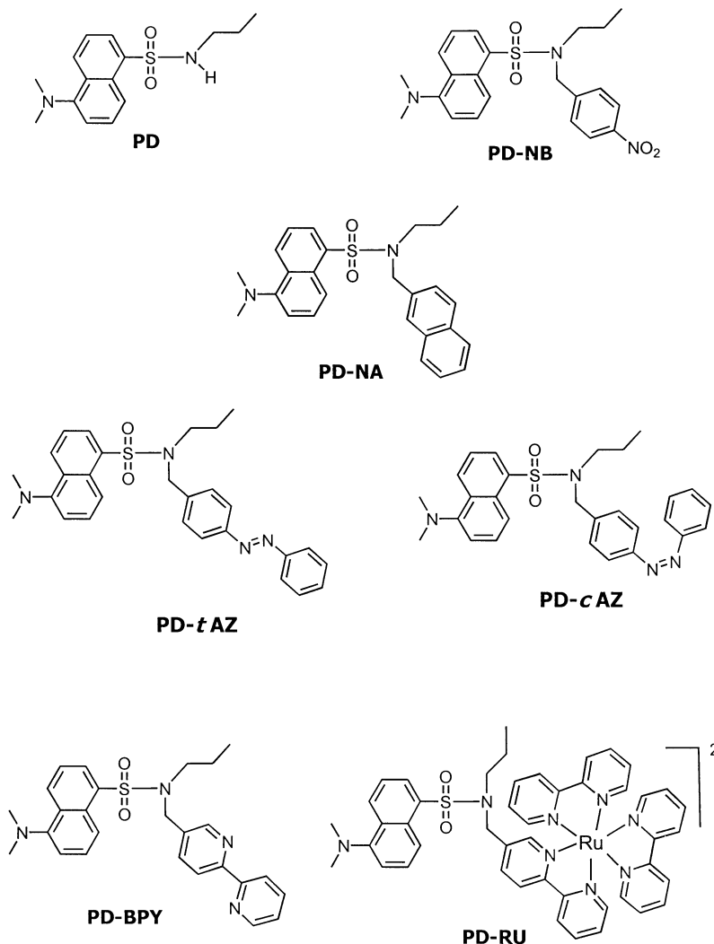
Scheme 1 5-Dimethylaminonaphthalene- N -propyl-1-sulfonamide molecule (PD) and the investigated dyads.
