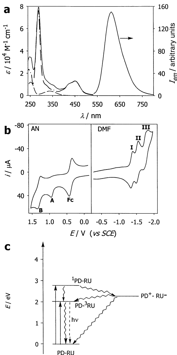
Fig. 7 (a) Absorption and emission spectra of the PD-RU dyad (full line) and absorption spectra of the PD (dashed line) and [\text{Ru}(\text{bpy})_3]^{2+} (dashed-dotted line) components in acetonitrile. (b) Cyclic voltammogram of the PD-RU dyad in acetonitrile-TBAPF 6 (anodic region) and dimethylformamide-TBAPF 6 (cathodic region) solutions. (c) Energy level diagram for the PD-RU dyad in acetonitrile solution at room temperature.
